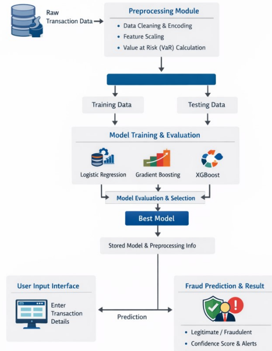
Fig 5.1: System Architecture
