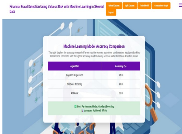
Fig 6.2: Algorithms trained
