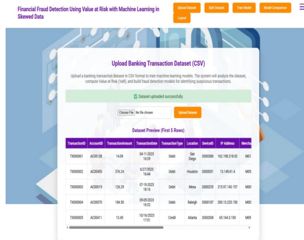
Fig 6.1: Dataset Uploaded
